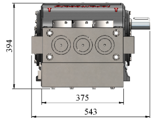
KDC BARE PUMP FRONT VIEW
