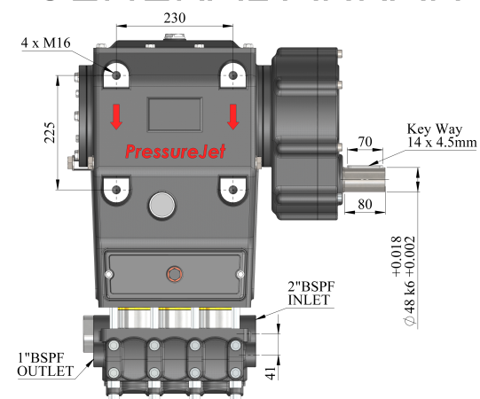
VA 57 BARE PUMP TOP VIEW
