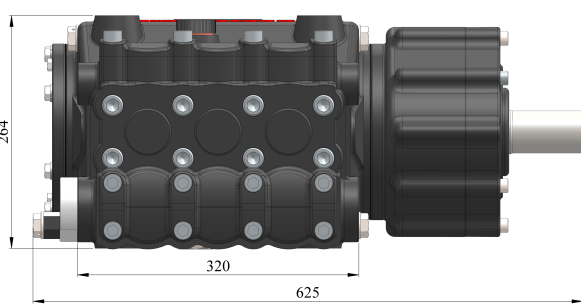
VA 57 BARE PUMP FRONT VIEW
