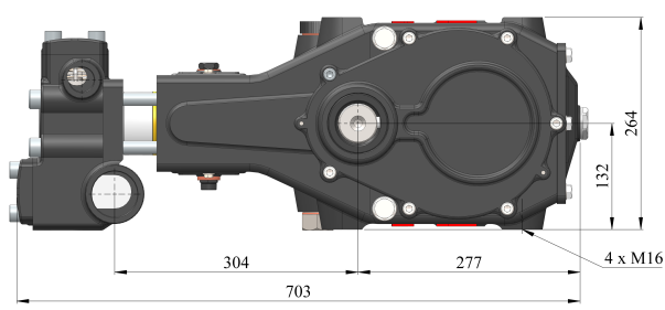
VA 57 BARE PUMP SIDE VIEW
